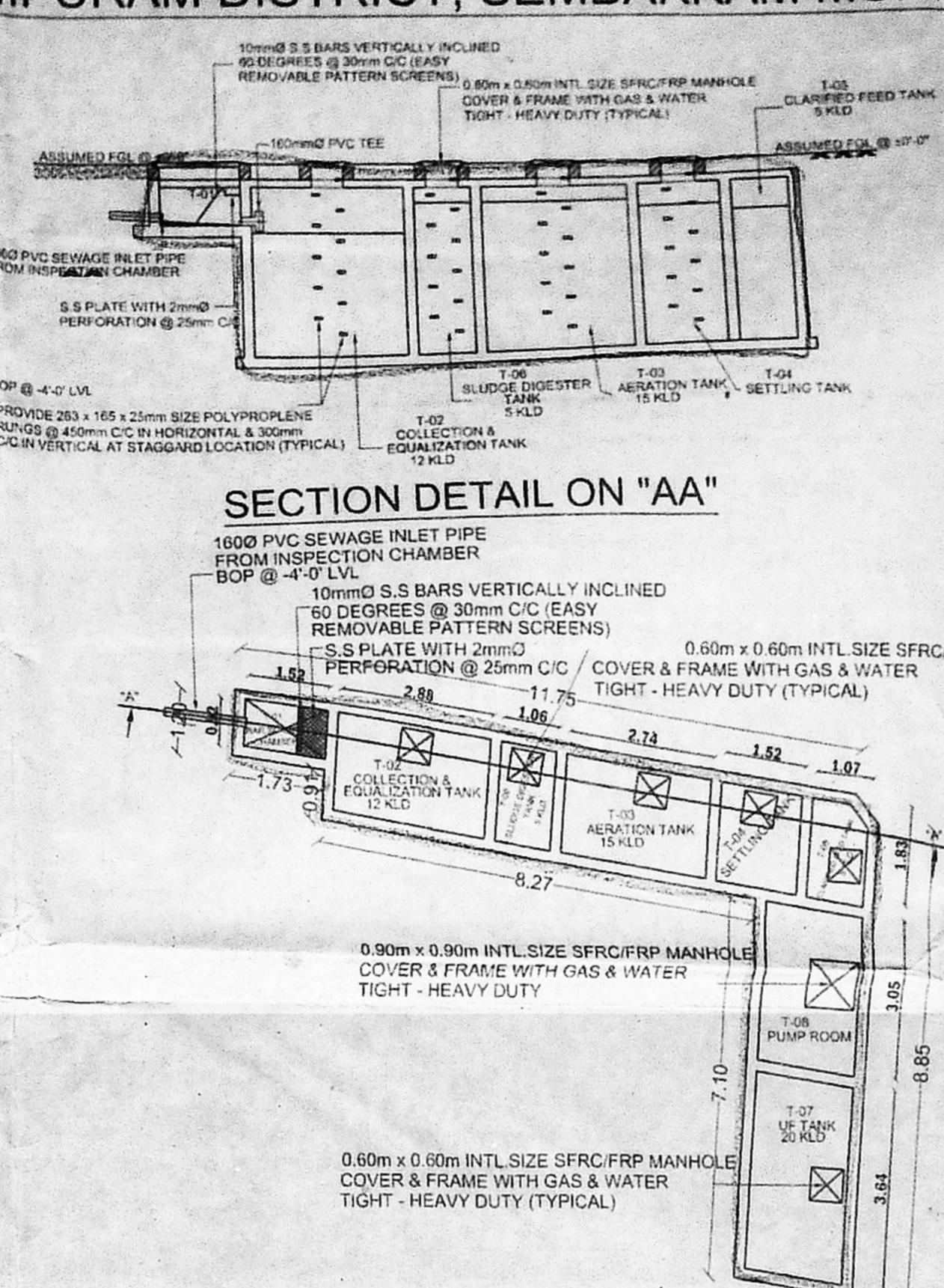
PLAN - SEWAGE TREATMENT PLANT AT BASE SLAB LEVEL - 25 KLD CAPACITY / PER DAY
